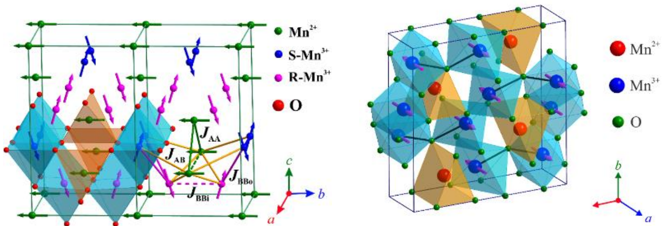
Fig. 25. Pressure-induced colossal enhancement of magnetic-ordering temperature in geometrically frustrated \text{Mn}_3\text{O}_4 oxide
